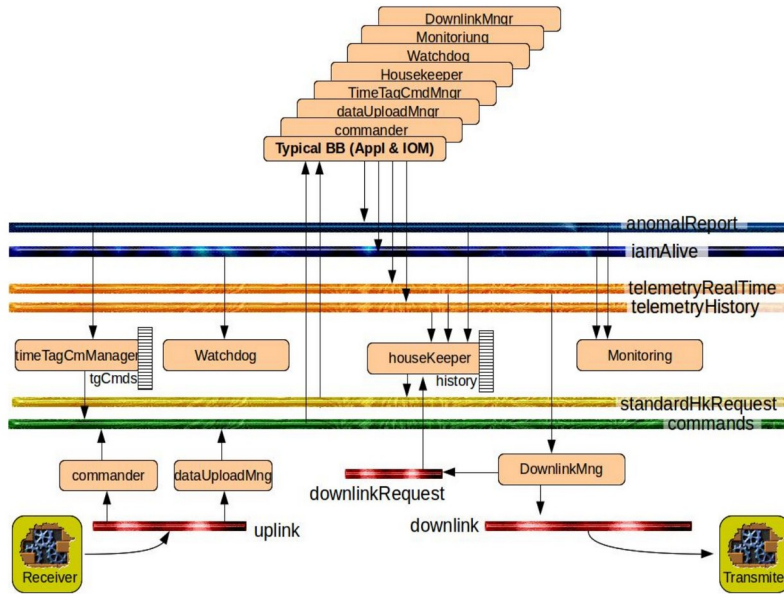
Figure 4: Typical Satellite Applications
