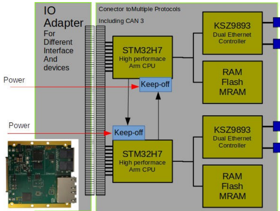
Figure 7: Dual Computer
