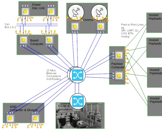
Figure 6: Dual-X structure of the avionics.
