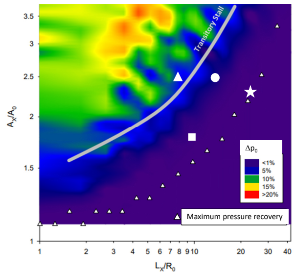
FIG 4. Flow regimes in straight-wall, three-dimensional quadratic diffusers, based on [12]
