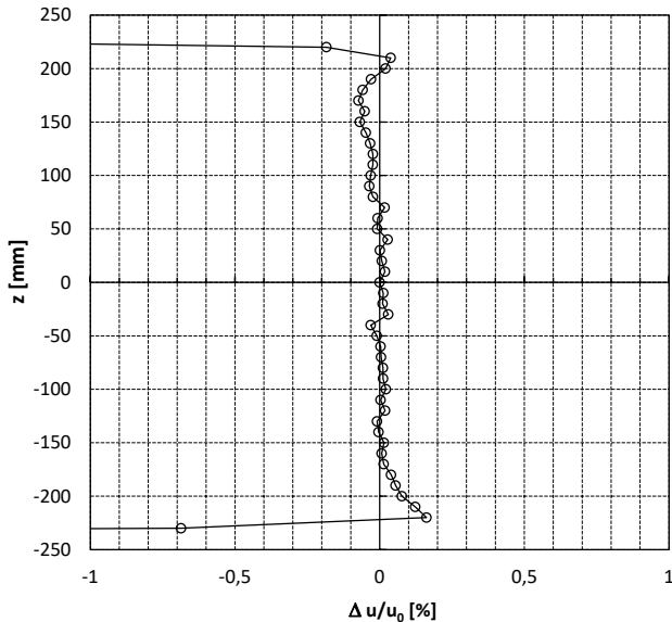
FIG 9. Relative vertical deviation of u_z from reference point at 40m/s at the test section centre
