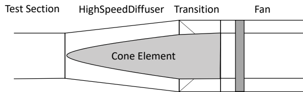
FIG 2. Cone element in high speed diffuser
