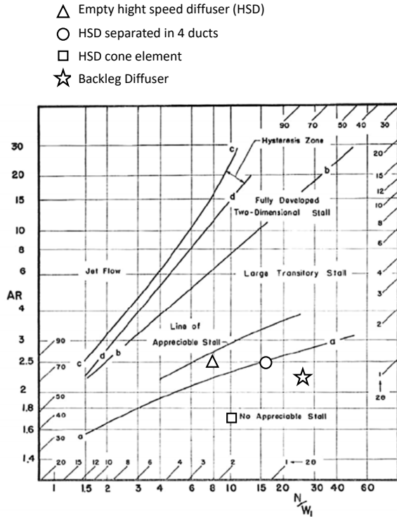
FIG 3. Flow regimes in straight-wall, two-dimensional diffusers, based on [11]
