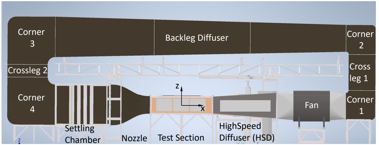
FIG 5. Sideview of wind tunnel
