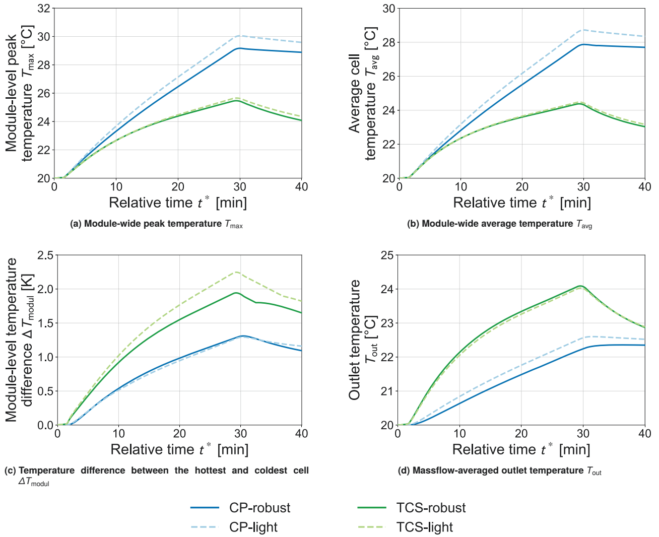
FIG 10. Thermal profiles of all cooling concepts over the relevant duration of the entire mission profile ( t^* = 0 min to 40 min).
