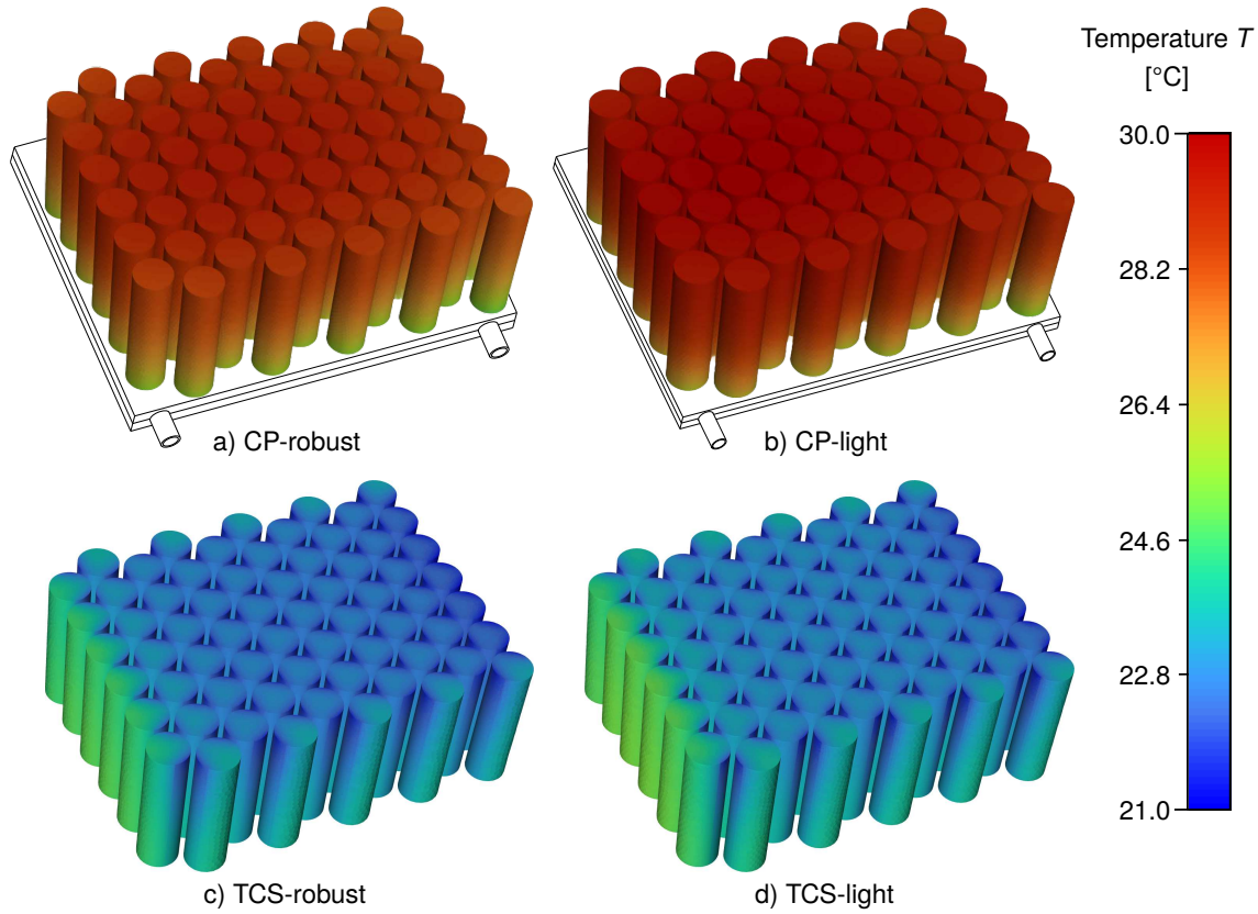
FIG 9. Surface temperatures of the battery cells at the end of the transient load profile (Nominal operation, t \approx 54 min). a) CP-robust, b) CP-light, c) TCS-robust, d) TCS-light.
