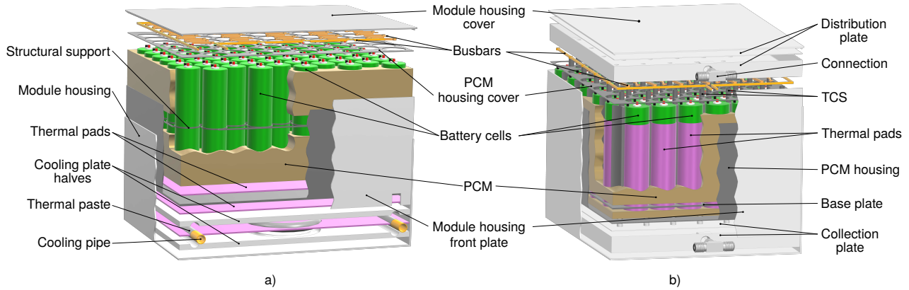
FIG 2. Exploded view of hybrid BTMS Design: a) CP-design: bottom cooling plate with intercellular PCM, b) TCS-design: intercellular TCS and bottom PCM.
