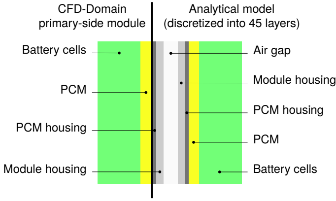
FIG 6. Boundary of numerically investigated geometry and analytical extension for propagation analysis.
