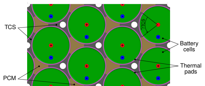
FIG 4. Top view of the internal layout of Design 2, illustrating the contact surface angle of the TCS, \gamma_{TCS} .
