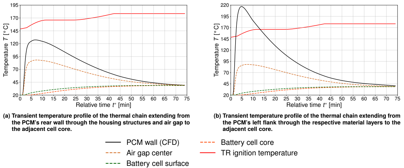
FIG 11. Transient temperature profiles obtained via the coupled transient one-dimensional multilayer post-processing analysis, evaluated against the SOC-dependent ignition temperature according to Amano et al. [23].
