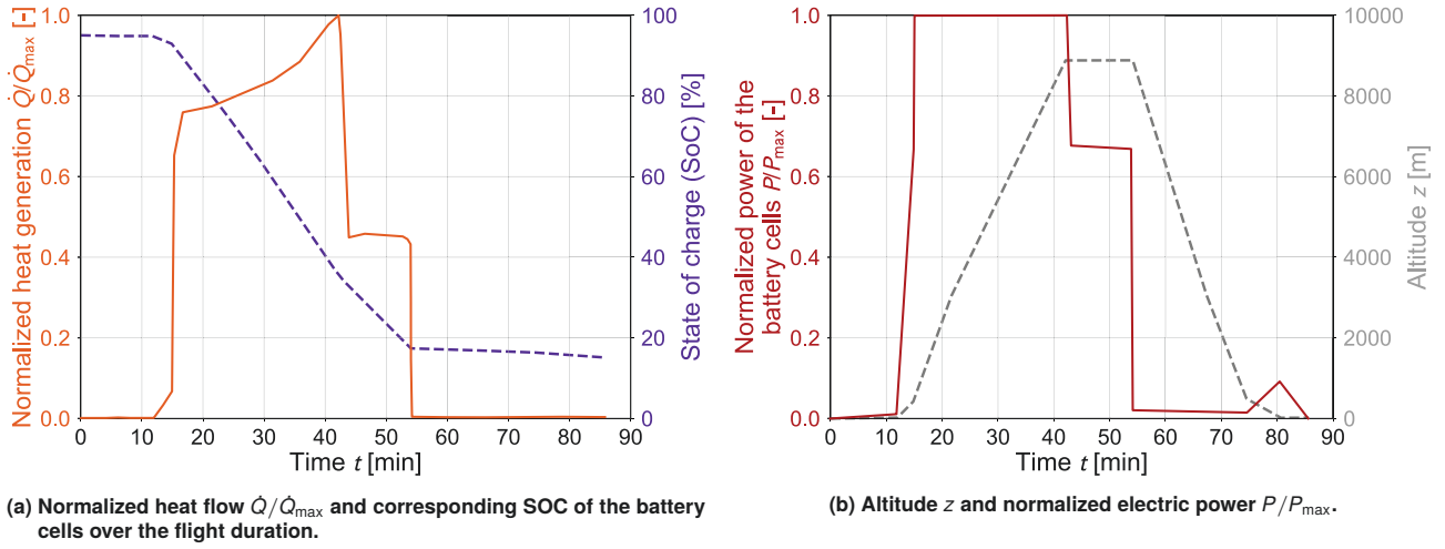
FIG 3. Investigated thermal profile corresponding to the flight profile of a fully electric regional passenger flight for 250 passengers with a range of 649 km originating from the DLR project EXACT2.
