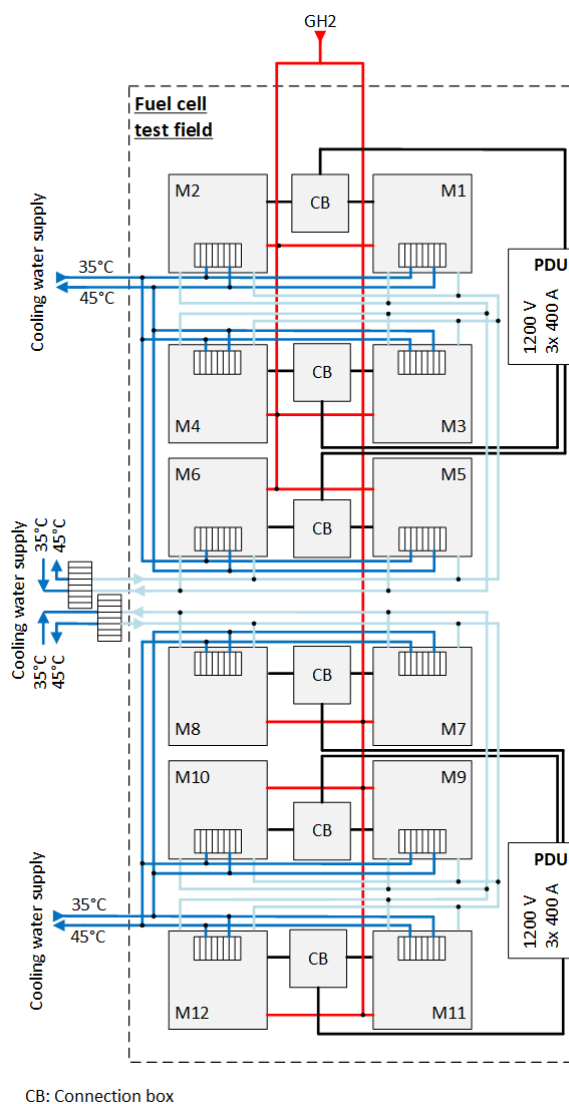
Figure 2 Overview of the system architecture of the BALIS 1 st generation fuel cell system integrated into the fuel cell test field; The numbers M1...12 denote the different fuel cell modules; dark blue: cooling water circuit, light blue: cold water circuit, red: hydrogen supply, black: HV DC system; The air supply and exhaust system is not depicted.
